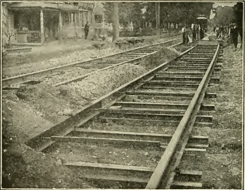
Fig. 232. Steel Tie and Tie-Rod Construction
